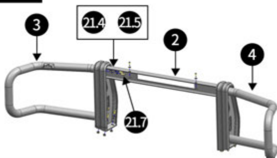
First, assemble the left and right wings and the middle crossbar together
