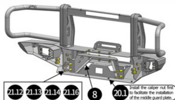
Assemble the Winch Support bracket and winch bracket together
