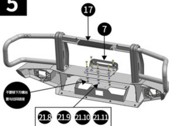
Attach the winch frame to the main body and install the LED light bar to the middle crossbar.
